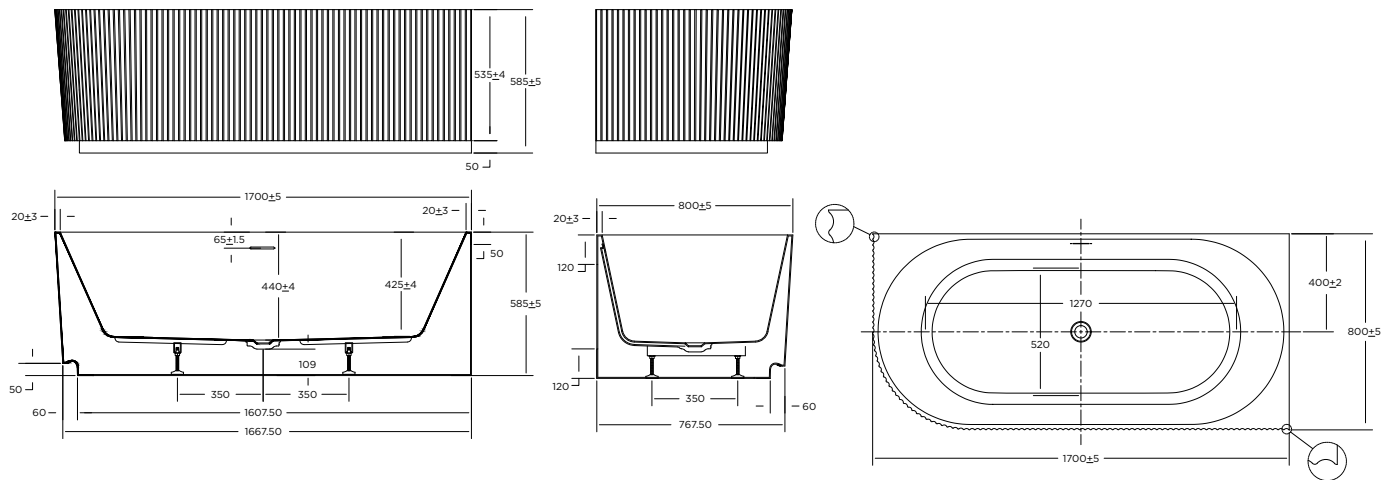
Technical Drawings
