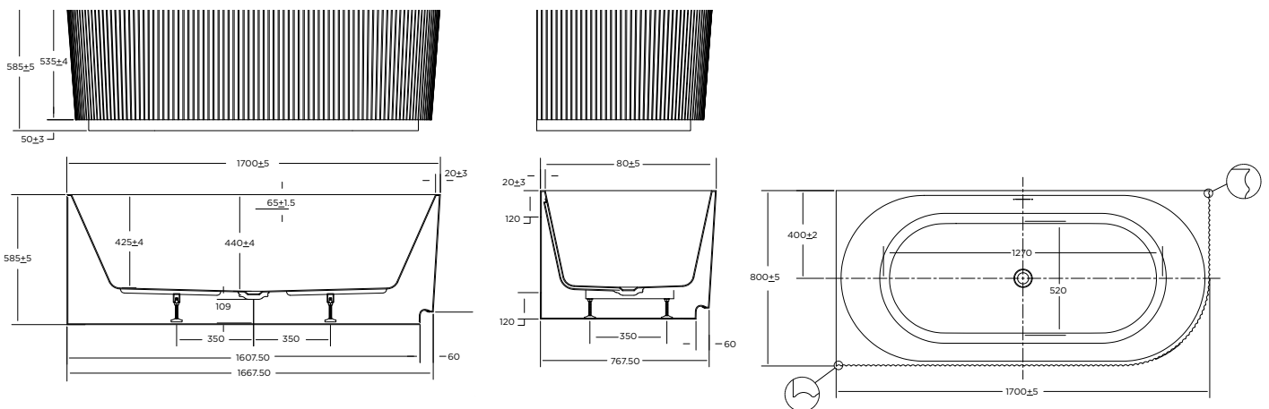
Technical Drawings
